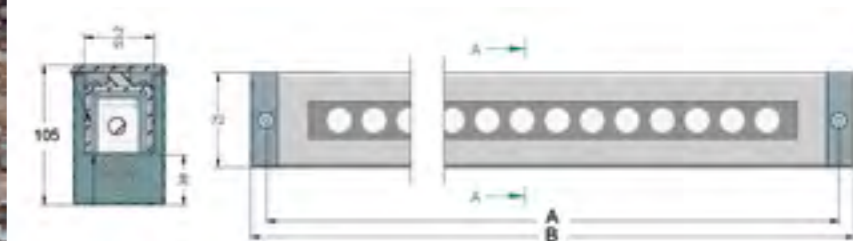
LINEAR FLOOR 16 LED : A 510 mm B 534mm LINEAR FLOOR 32 LED : A 1020mm B 1070mm
